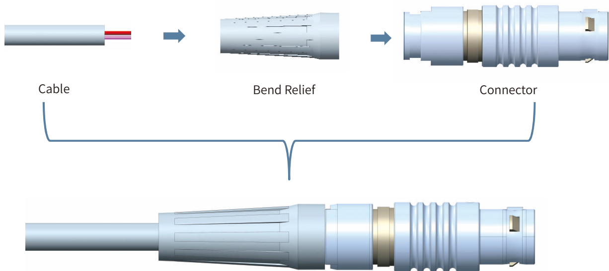
Assembly Drawing
